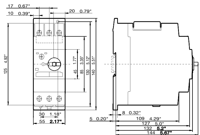
MS450-40...MS450-50, MS451-16...MS451-50
