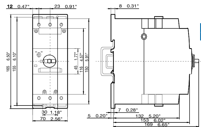
MS495-40...MS495-100, MS496-40...MS496-100
